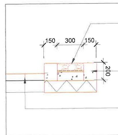
SECTION X-X
