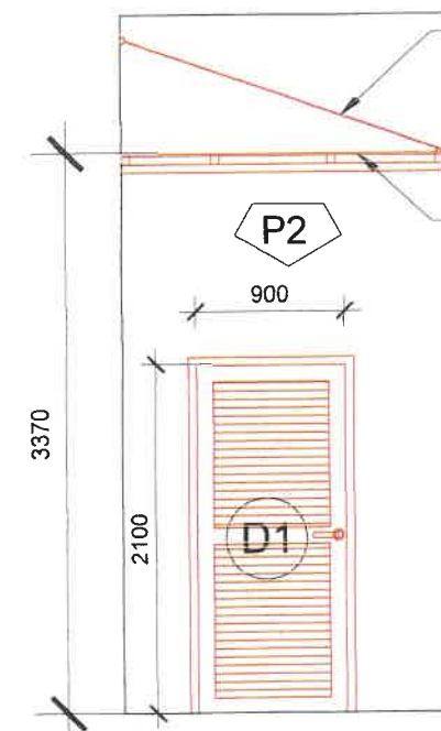
VIEW 'C' (VEW)
