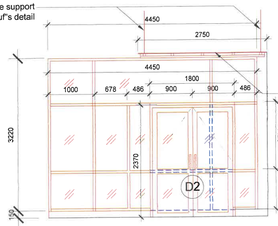
VIEW 'A' (VEW)
